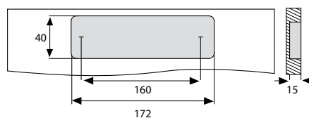
MECANIZADO PUERTA ROATING DETAILS
